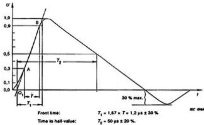
Figure 2 - Waveform of open-circuit voltage (1,2/50 \mu s) (waveform definition according to IEC 60-1)
